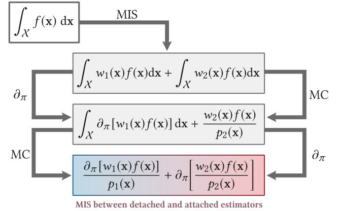
Fig. 6. The decision of whether to attach or detach a sampling technique and its MIS weight can be made separately for each technique, as illustrated by this derivation sketch.
