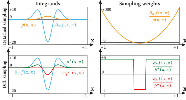
Fig. 7. 1D examples of custom differential samplers. Top row: The wrapped normal distribution p is ill-suited for sampling its derivative \partial_\pi f = \partial_\pi p and produces large weights. Bottom row: the densities p^+ and p^- are proportional to the positive and negative regions of \partial_\pi f and produce constant sampling weights that reduce the variance of the estimator.
