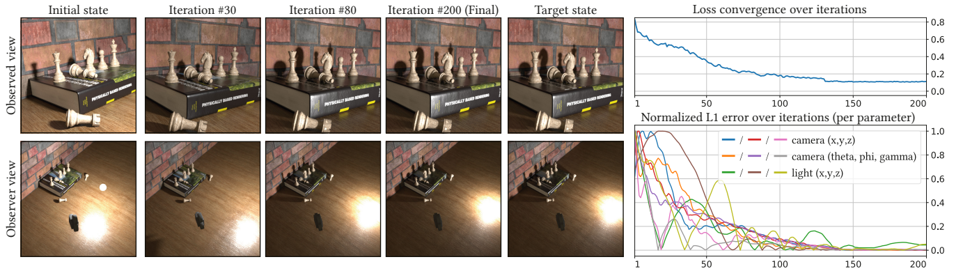
Fig. 15. 6D camera pose and light position estimation in a scene with complex light transport involving soft shadows and glossy interreflections. Top: Camera view at different steps during optimization. Bottom: Visualization of the scene from the top at the same steps (camera shown as an actual object). Right: Convergence of the loss and error plots of the 9 parameters that are jointly optimized. The supplemental video shows an animated version of this result.
