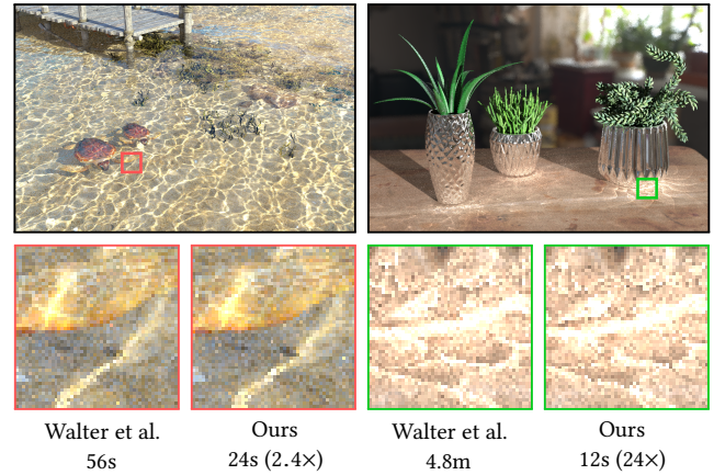
Fig. 9. Equal sample comparison (20 spp) between our pruning strategy and the pruning strategy proposed by Walter et al. [2009]. The previous strategy performs well for refractive caustics (left) but poorly for reflection. Our precomputed pruning hierarchy supports faster specular triangles queries and adaptive stochastic pruning that make SNEE practical for both types of specular sub-paths. Times do not include our precomputation passes, which took 15s (left) and 20s (right). Specular interactions inside selected triangles have been sampled using our techniques in all images.
