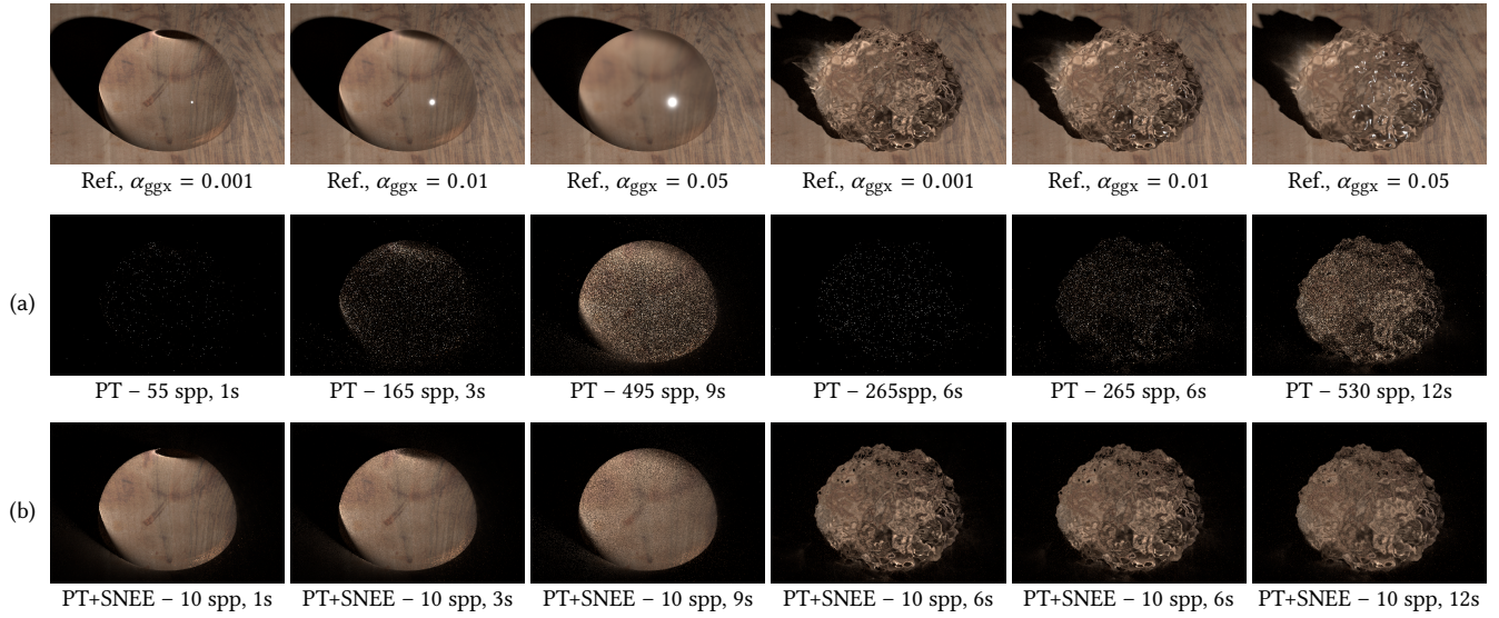
Fig. 10. Various scenes rendered with equal sample counts for PT+SNEE (b, our), and equal time comparison against standard path tracing (a). These results show how the cost of SNEE increases with the roughness of the material and the complexity of the caustics. Images in (a) and (b) only contain contributions from light paths that can be sampled by SNEE.
